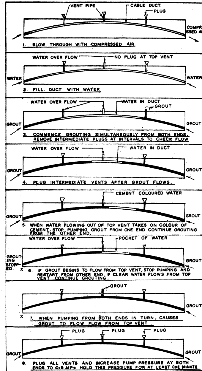
Fig. 9. Procedure for grouting of cables draped downwards
