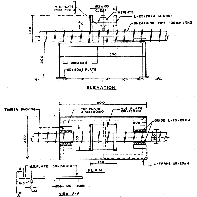
Fig. 6. Transverse load rating test
