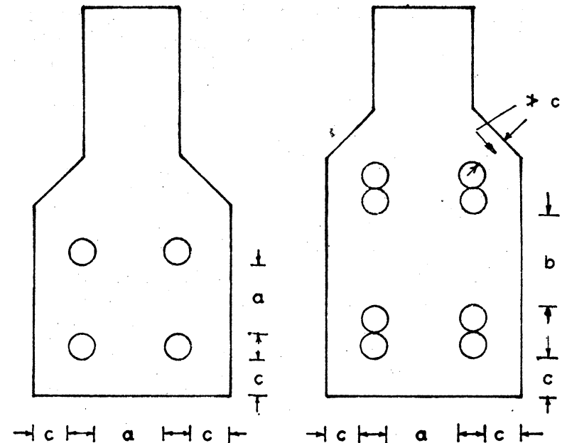
a, b \leq 50 mm or 10 mm in excess of the largest size of aggregate used or diameter of duct whichever is greater e \leq 50 mm, the value of c to be increased by 10 mm for severe exposure conditions.
